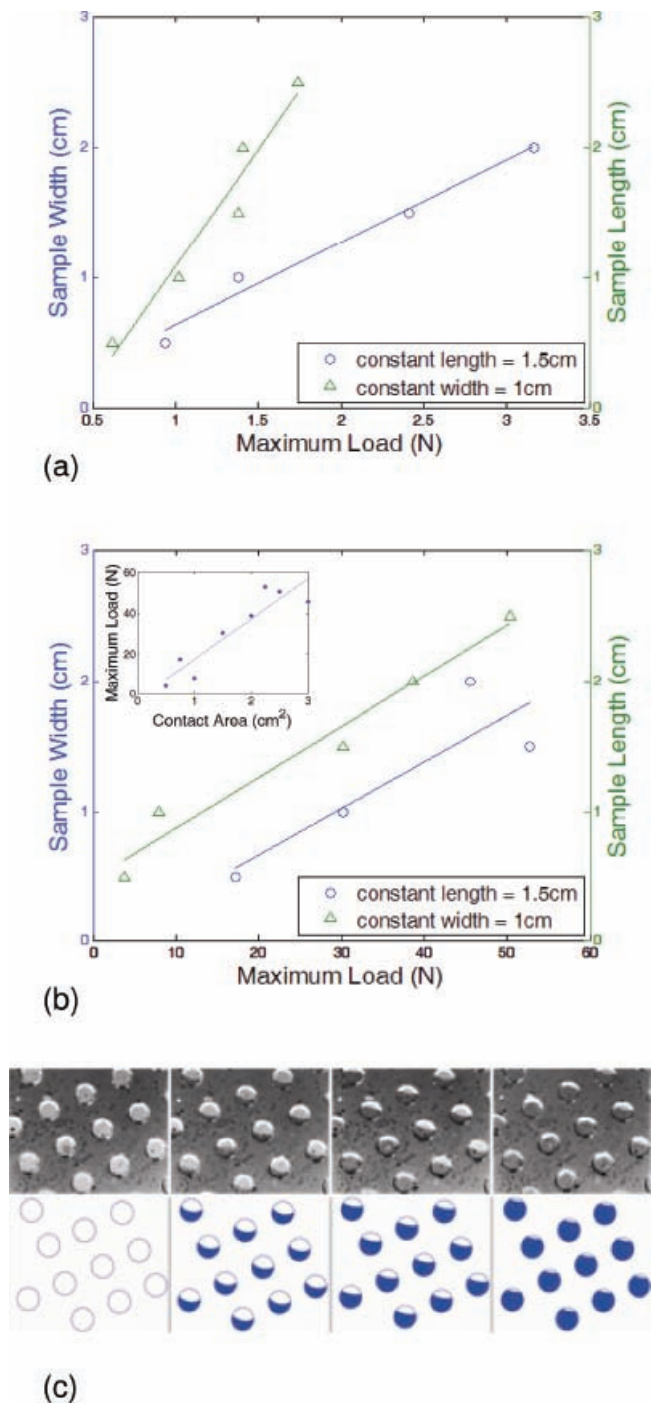
Figure 3. a,b) Maximum shear force dependence on sample width and length for (a) an unpatterned PDMS film and (b) a micropatterned PDMS film. Inset: Shear force scales linearly with area for patterned samples. c) Still frames (enhanced contrast) from top-down video of an array of the PDMS microstructures under pure shear. The microstructures are adhered to a glass slide, which is being steadily moved in the upward (slightly right) direction. At the critical shear load, a stress concentration at the edge opposite the direction of the shear force causes an interfacial crack to propagate across each microstructure in the array simultaneously. Crack propagation can be seen by the color contrast between adhered and detached surfaces. An illustrative sequence of images is provided for clarity.
